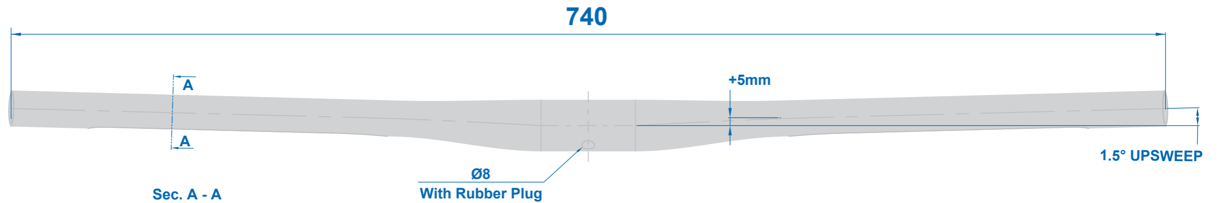
FRONT VIEW
