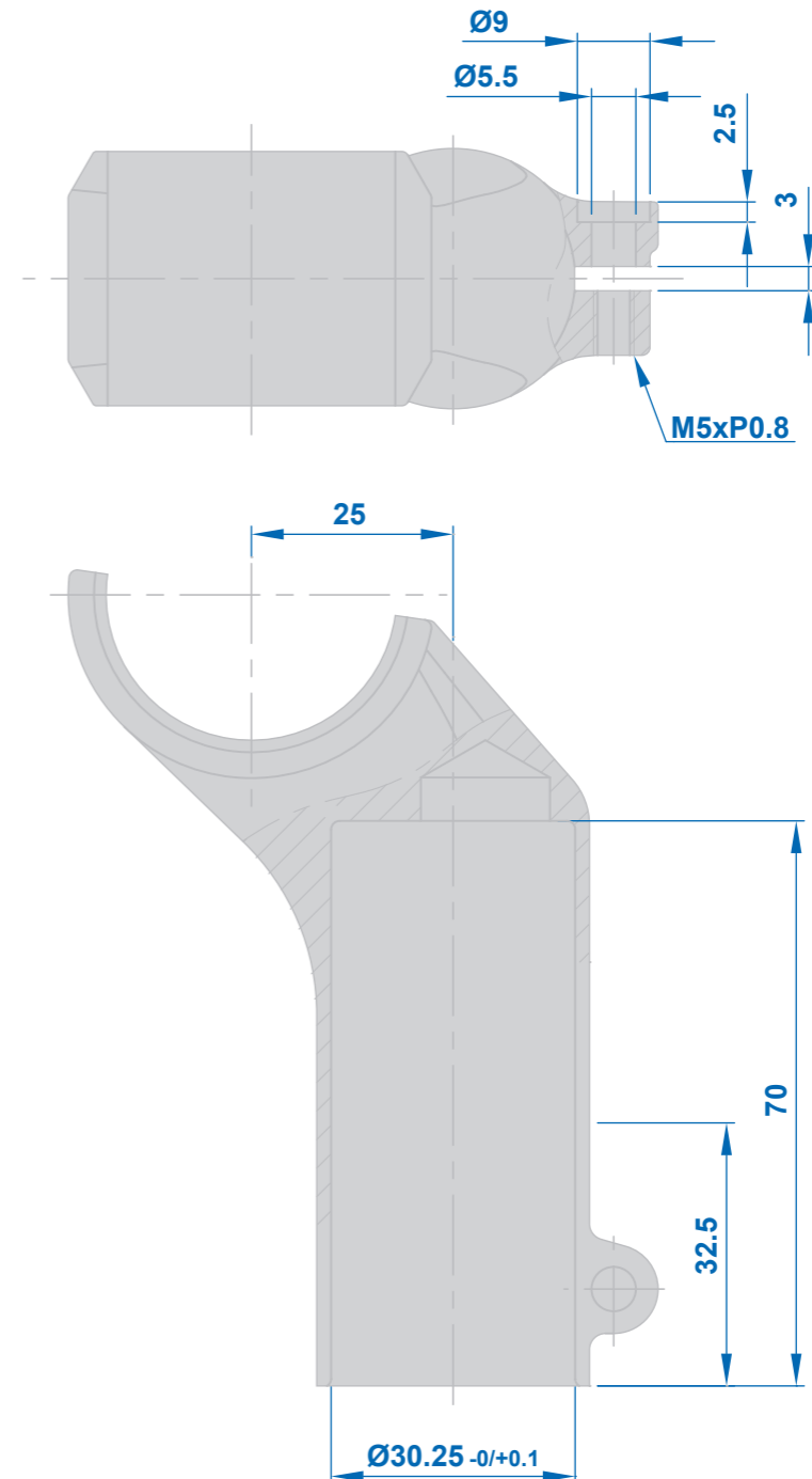
25mm OFFSET / 70mm x 30.25 DIAMETER
